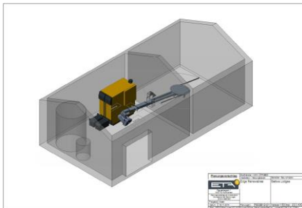
The layout of Bettws Hall plant room
